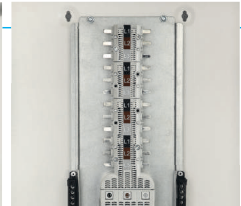
Completely insulated bus bars guarantee safety from severe shocks
