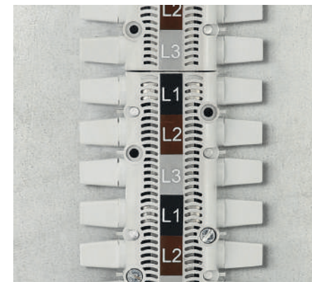
Plastic caps for complete insulation of unused connections
